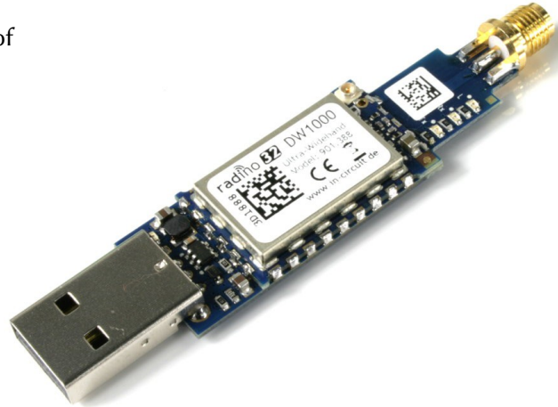
radino USB-Stick (with radino 32 DW1000)
