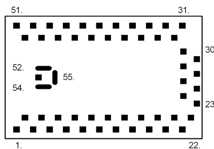
Footprint deRFmega128-22M10
