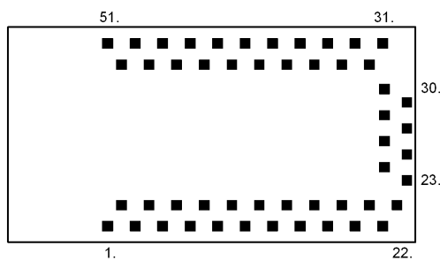
Footprint deRFmega128-22M00
