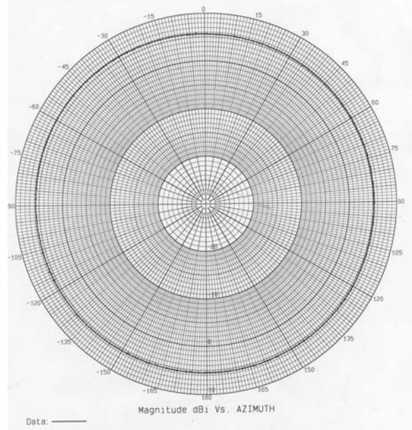
LMR Series @ 1900 MHz – Azimuth Plot
