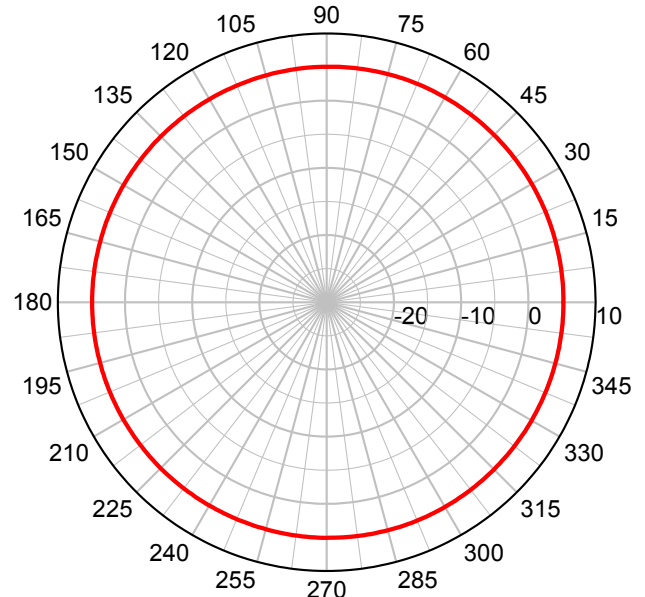
MRM3-5500 Series – Azimuth Plot
