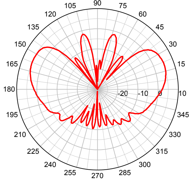
MRM3-5500 Series – Elevation Plot
