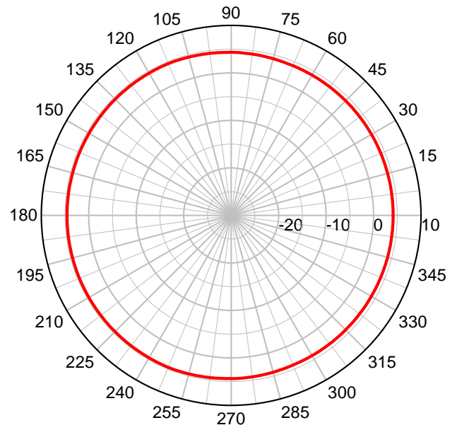
MGRM at 2100 MHz – Azimuth Plot
