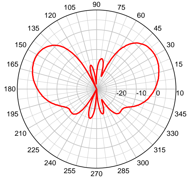
MGRM at 2100 MHz – Elevation Plot
