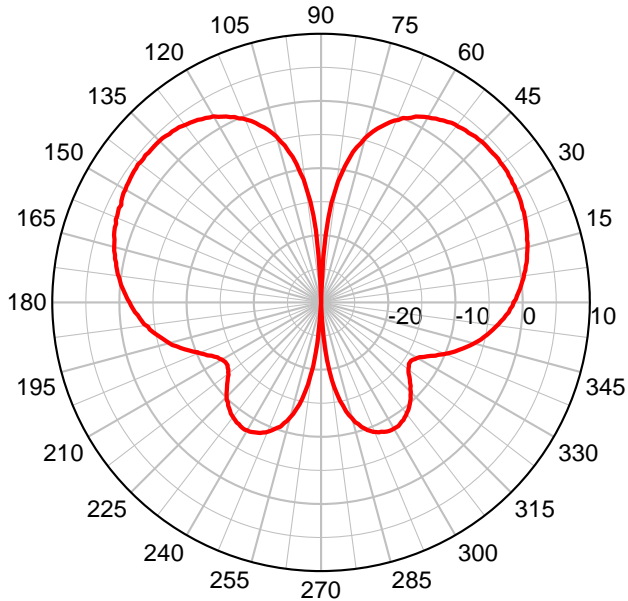
MGRM at 900 MHz – Elevation Plot
